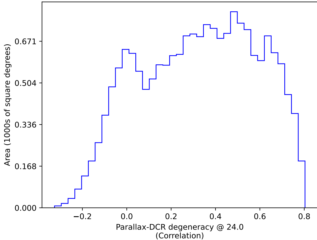
too_elab_2yr_r128_d3_ugrizy_v3.4_10yrs WFD: Parallax-DCR degeneracy @ 24.0
