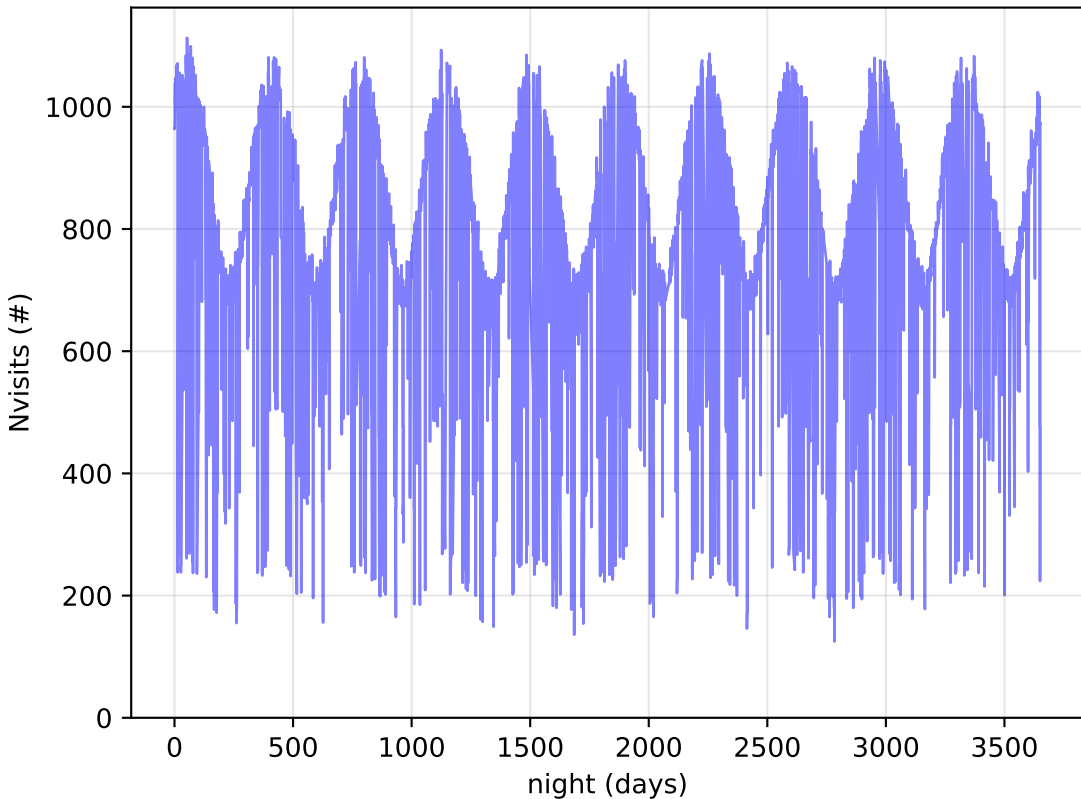
too_elab_2yr_r128_d3_ugrizy_v3.4_10yrs All visits: Nvisits
