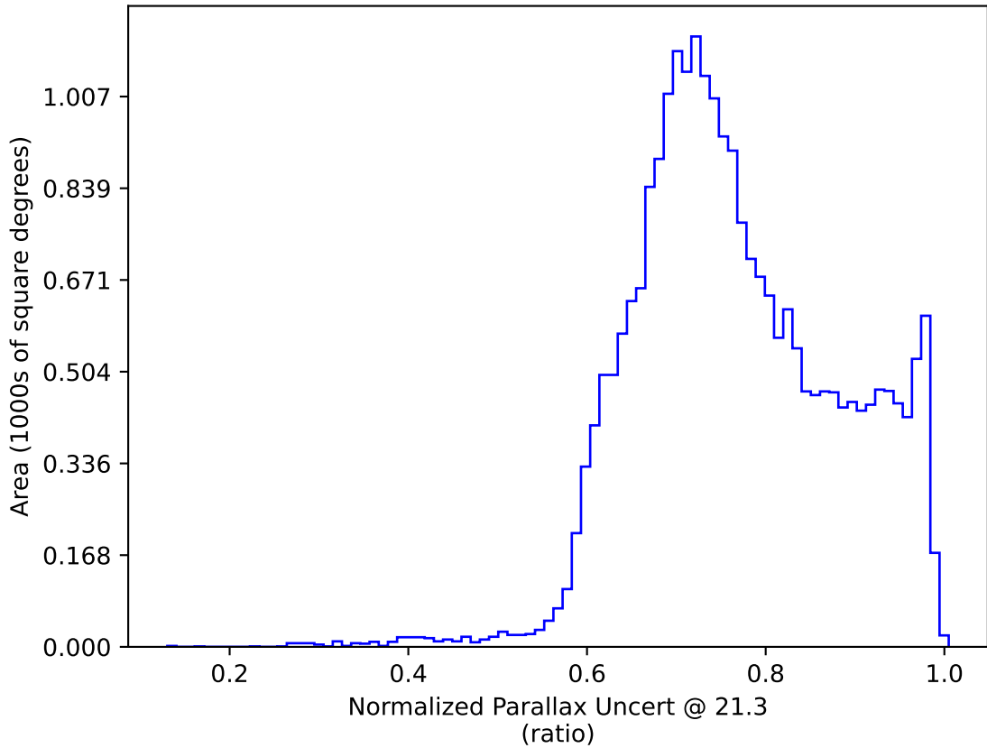
too_elab_2yr_r128_d3_ugrizy_v3.4_10yrs All sky y band only: Normalized Parallax Uncert @ 21.3
