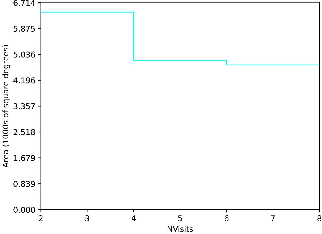
too_elab_2yr_r128_d3_ugrizy_v3.4_10yrs Yr 3-4 u band: NVisits
