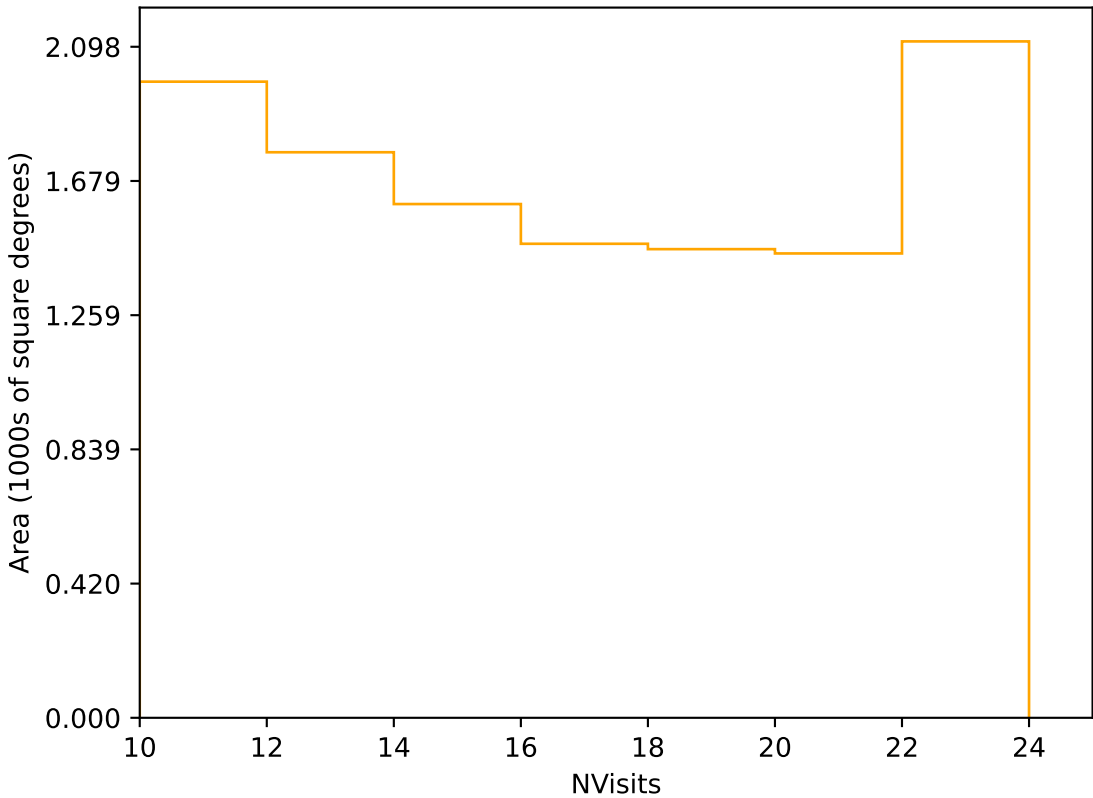
too_elab_2yr_r128_d3_ugrizy_v3.4_10yrs Yr 3-4 r band: NVisits
