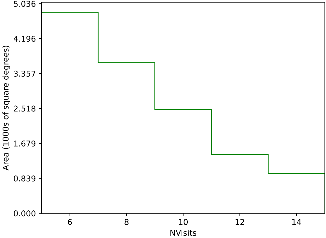
too_elab_2yr_r128_d3_ugrizy_v3.4_10yrs Yr 3-4 g band: NVisits
