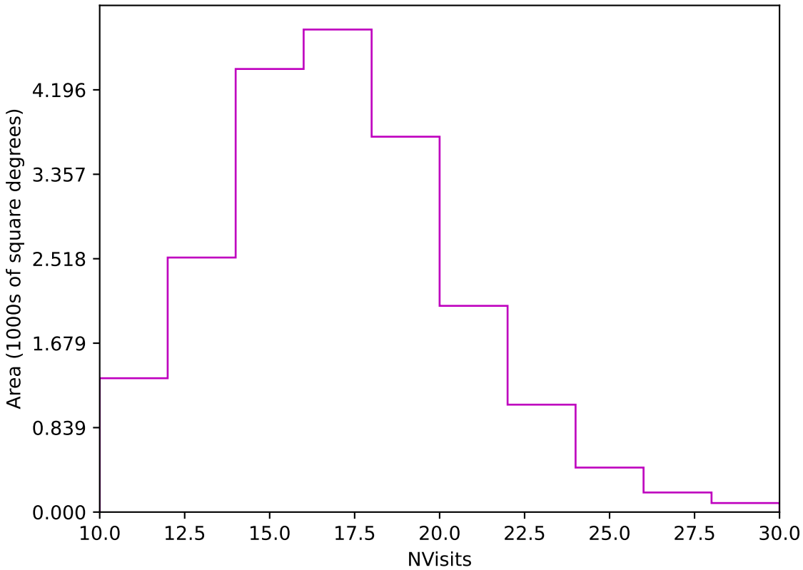
too_elab_2yr_r128_d3_ugrizy_v3.4_10yrs Yr 1 z band: NVisits
