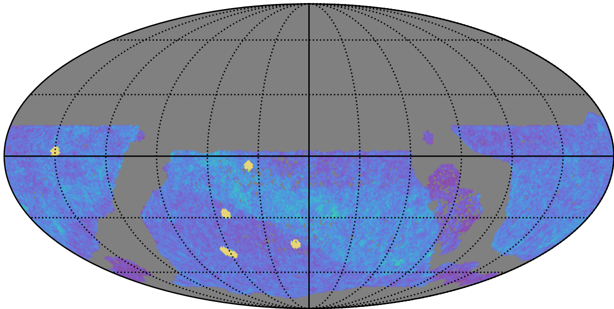
too_elab_2yr_r128_d3_ugrizy_v3.4_10yrs WFD z band: NVisits
