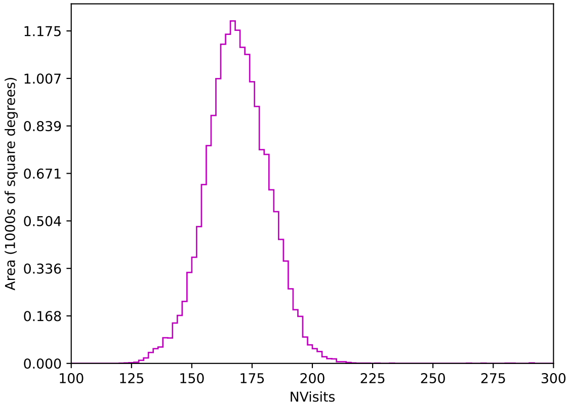
too_elab_2yr_r128_d3_ugrizy_v3.4_10yrs WFD z band: NVisits
