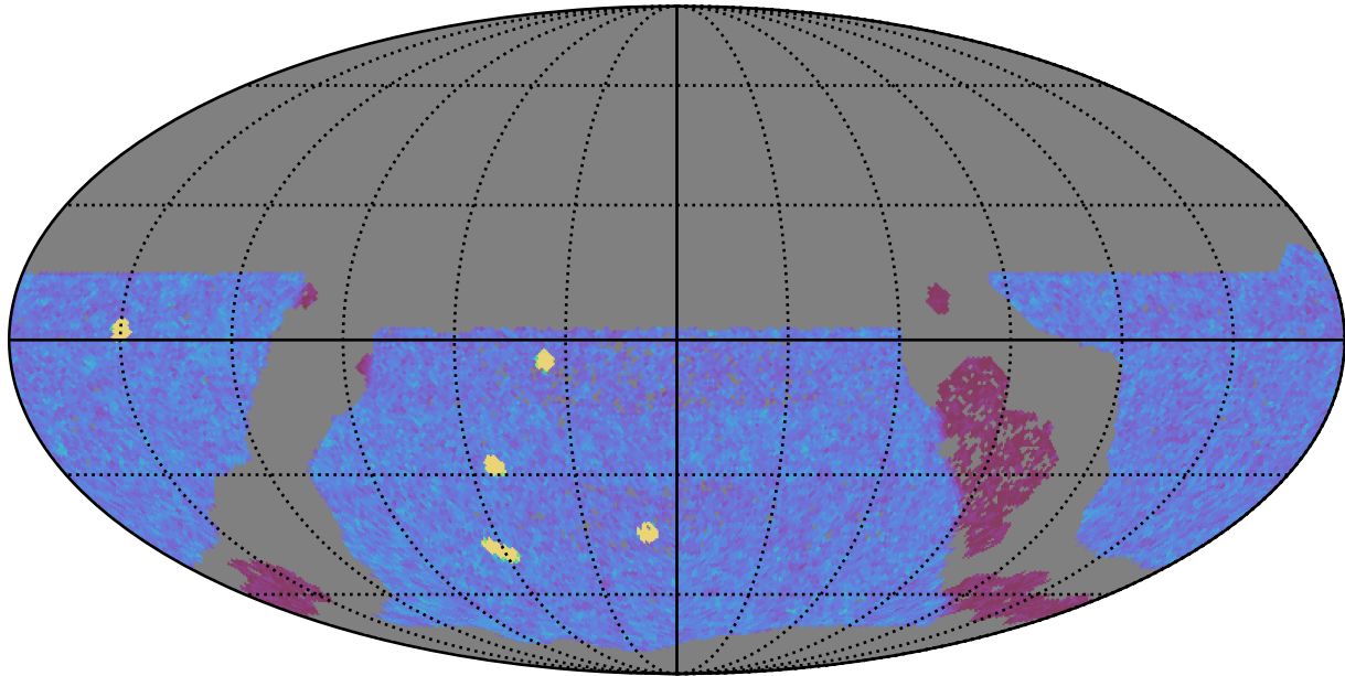
too_elab_2yr_r128_d3_ugrizy_v3.4_10yrs WFD y band: NVisits
