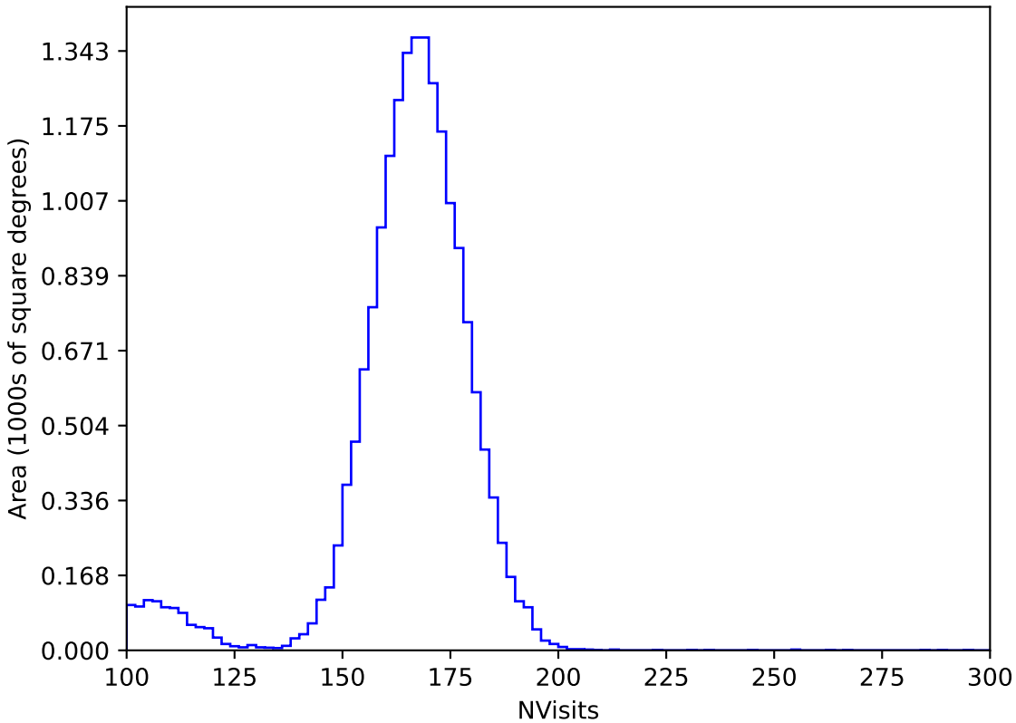
too_elab_2yr_r128_d3_ugrizy_v3.4_10yrs WFD y band: NVisits
