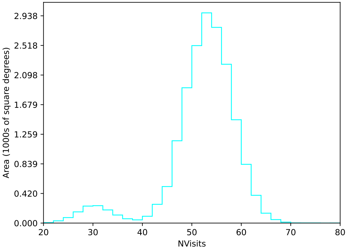
too_elab_2yr_r128_d3_ugrizy_v3.4_10yrs WFD u band: NVisits
