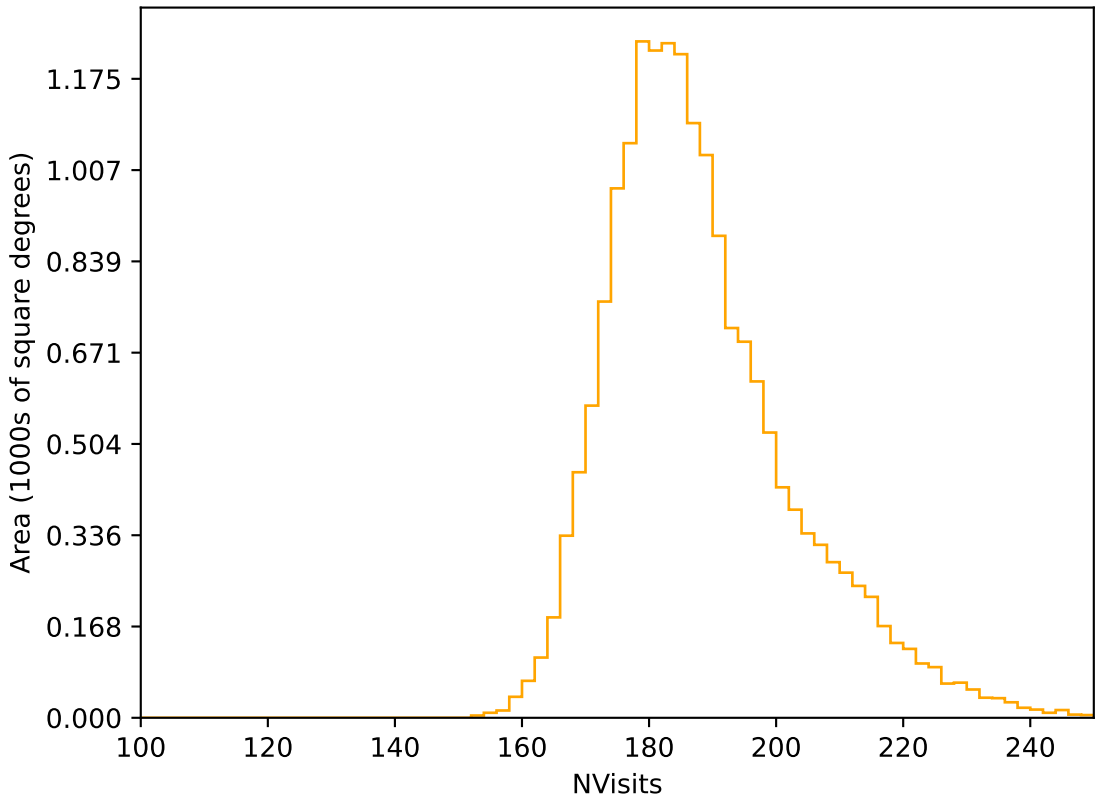
too_elab_2yr_r128_d3_ugrizy_v3.4_10yrs WFD r band: NVisits
