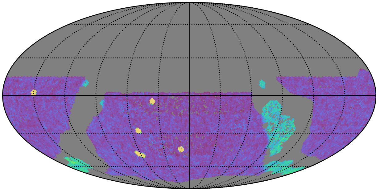
too_elab_2yr_r128_d3_ugrizy_v3.4_10yrs WFD g band: NVisits
