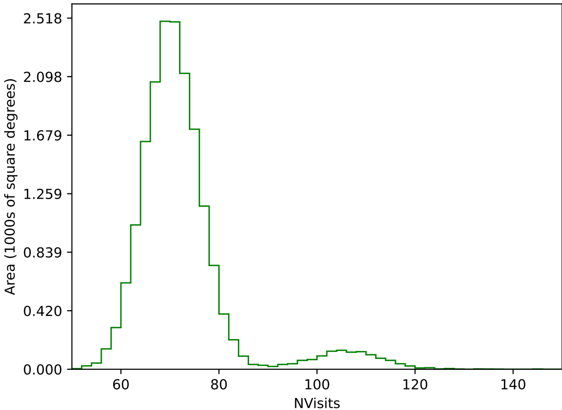
too_elab_2yr_r128_d3_ugrizy_v3.4_10yrs WFD g band: NVisits
