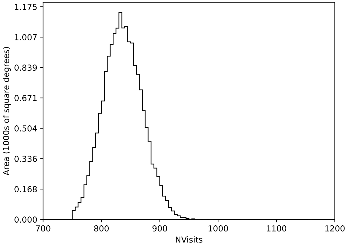
too_elab_2yr_r128_d3_ugrizy_v3.4_10yrs WFD all bands: NVisits
