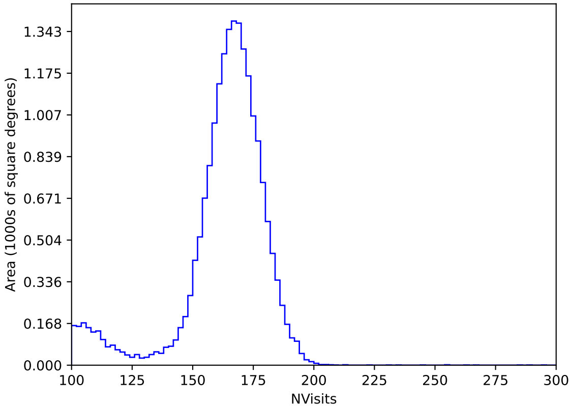
too_elab_2yr_r128_d3_ugrizy_v3.4_10yrs All sky y band: NVisits
