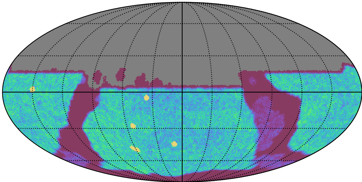
too_elab_2yr_r128_d3_ugrizy_v3.4_10yrs All sky u band: NVisits
