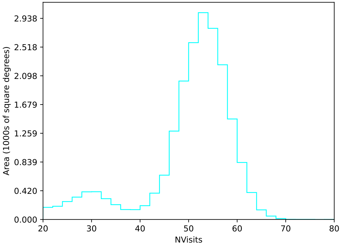
too_elab_2yr_r128_d3_ugrizyv3.4_10yrs All sky u band: NVisits
