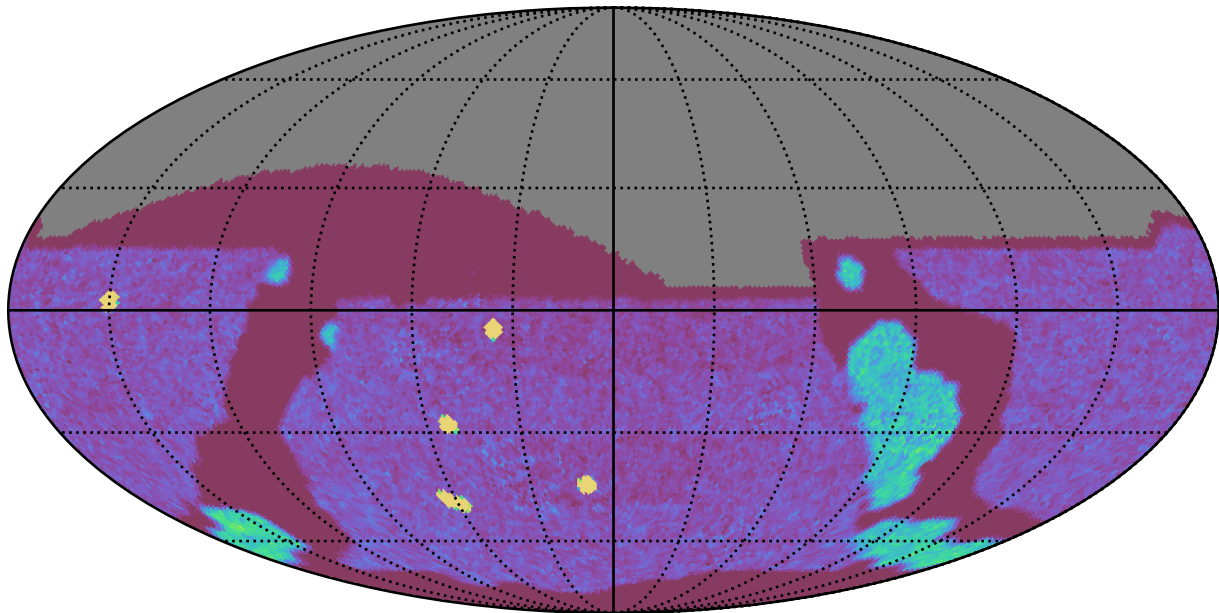
too_elab_2yr_r128_d3_ugrizy_v3.4_10yrs All sky g band: NVisits
