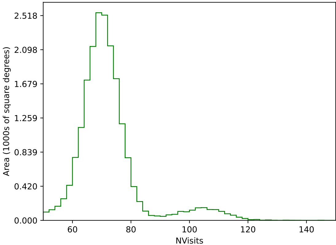
too_elab_2yr_r128_d3_ugrizy_v3.4_10yrs All sky g band: NVisits
