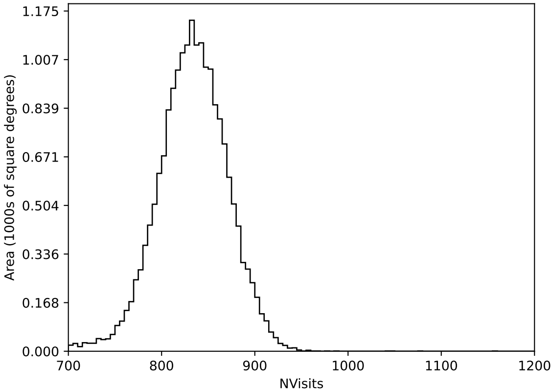
too_elab_2yr_r128_d3_ugrizy_v3.4_10yrs All sky all bands: NVisits
