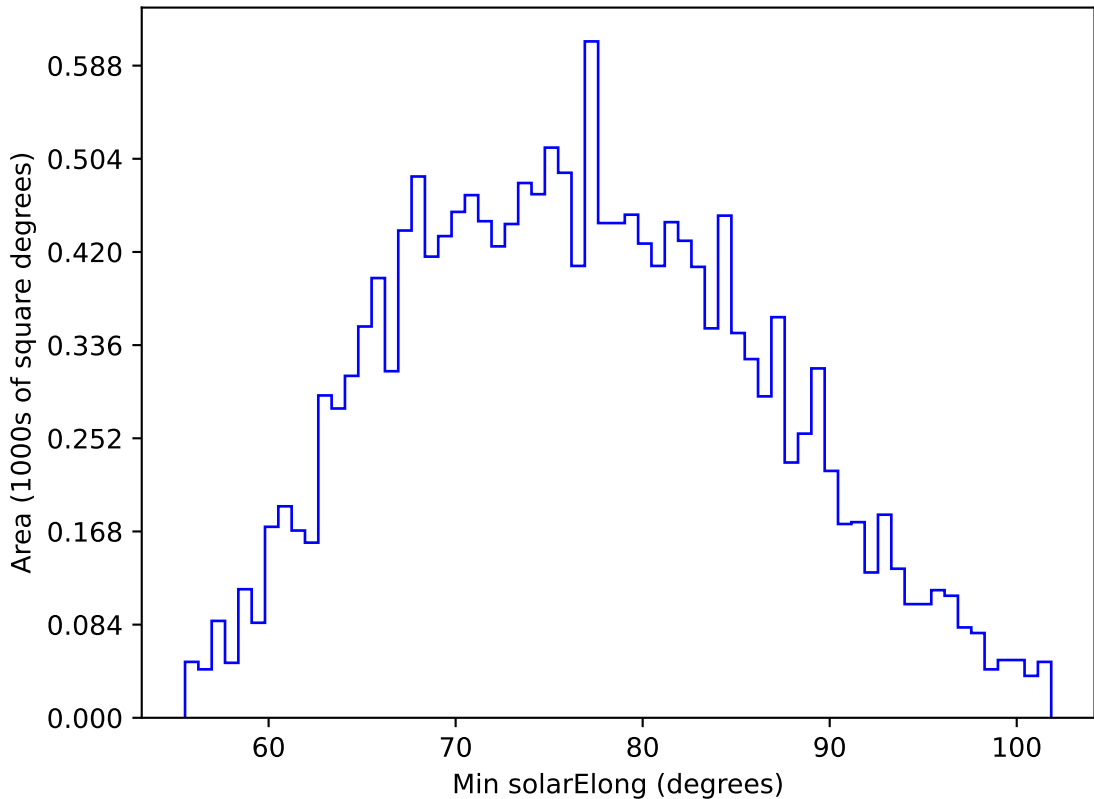
too_elab_2yr_r128_d3_ugrizy_v3.4_10yrs WFD u band: Min solarElong
