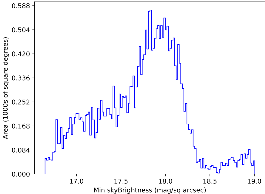
too_elab_2yr_r128_d3_ugrizy_v3.4_10yrs Yr 1 all bands: Min skyBrightness
