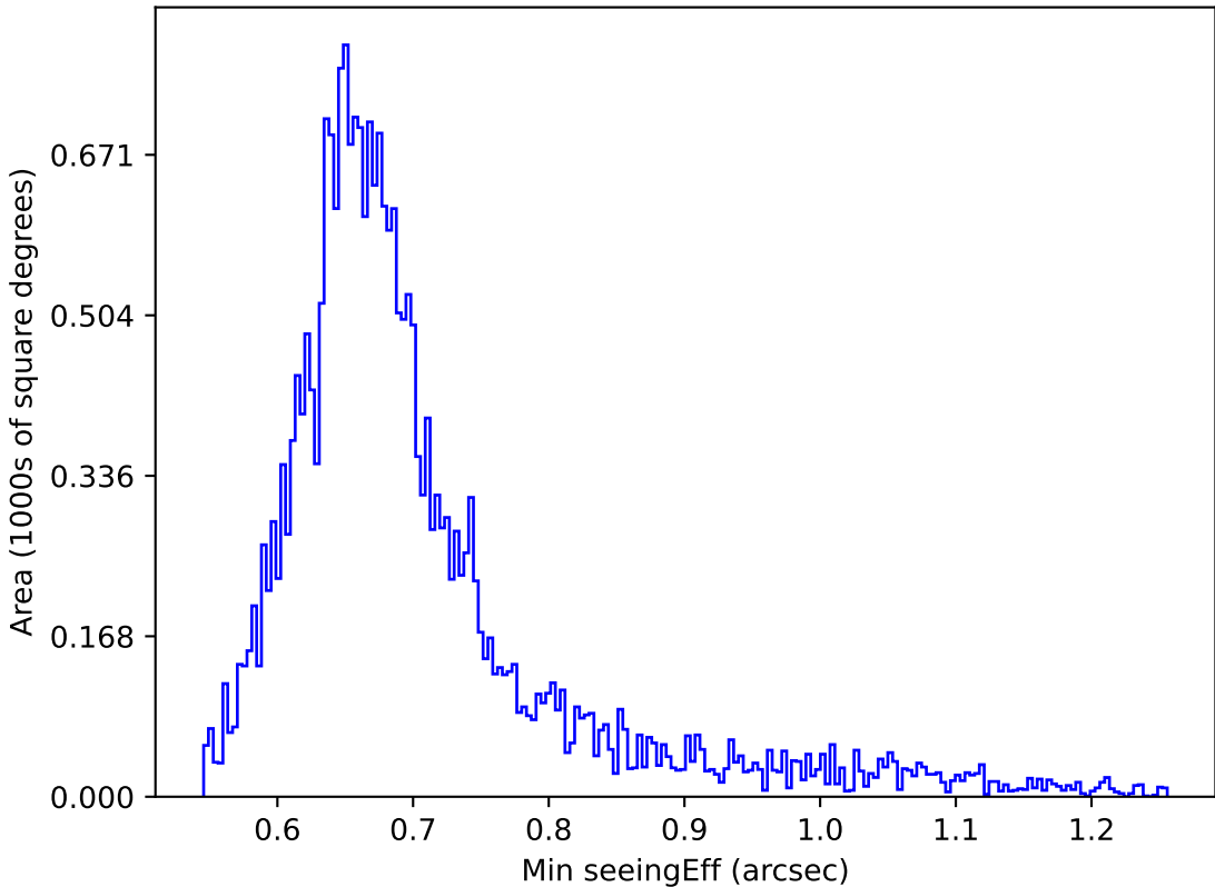
too_elab_2yr_r128_d3_ugrizy_v3.4_10yrs Yr 1 i band: Min seeingEff
