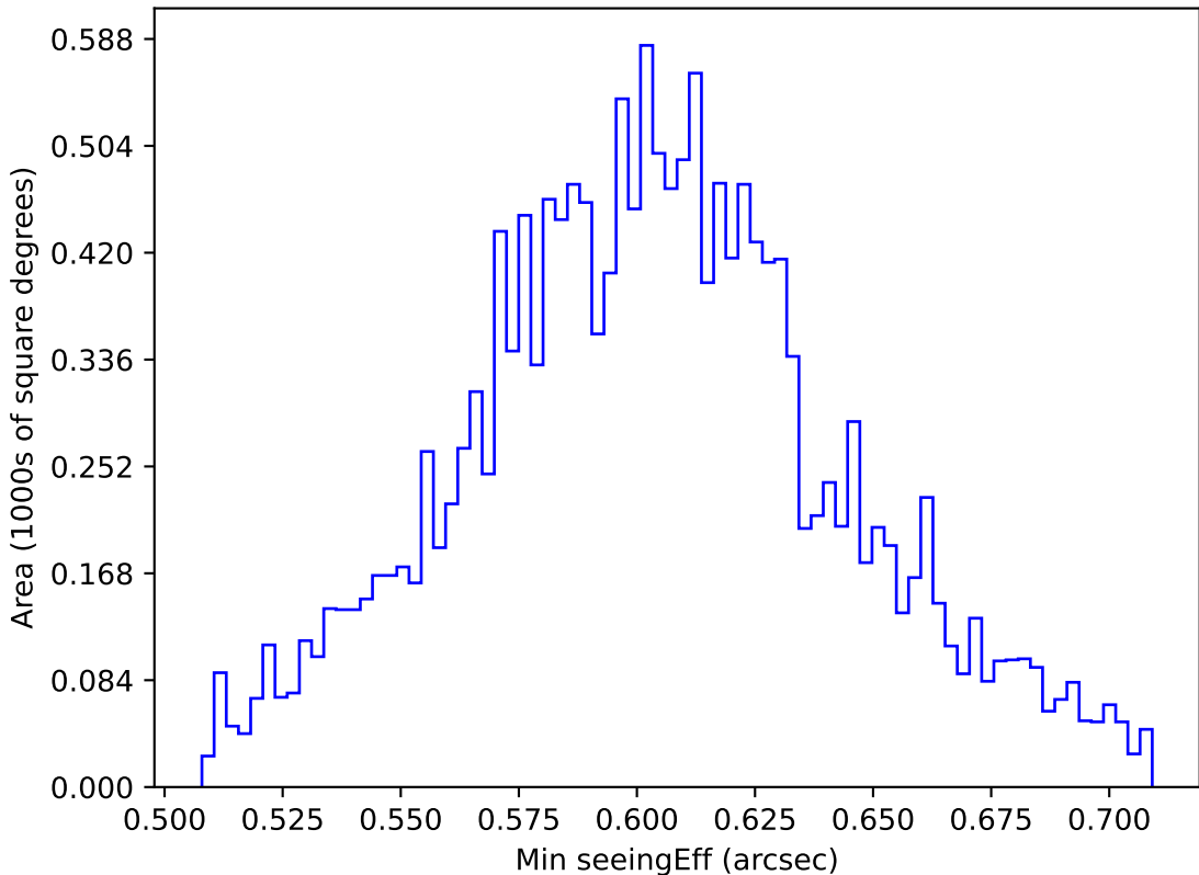
too_elab_2yr_r128_d3_ugrizy_v3.4_10yrs WFD i band: Min seeingEff
