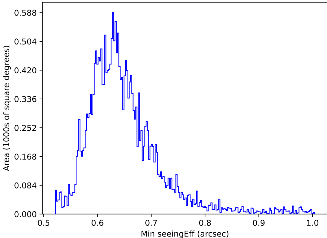
too_elab_2yr_r128_d3_ugrizy_v3.4_10yrs All sky y band: Min seeingEff
