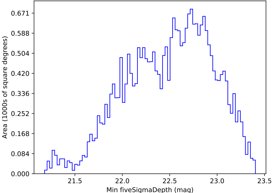
too_elab_2yr_r128_d3_ugrizy_v3.4_10yrs All sky r band: Min fiveSigmaDepth
