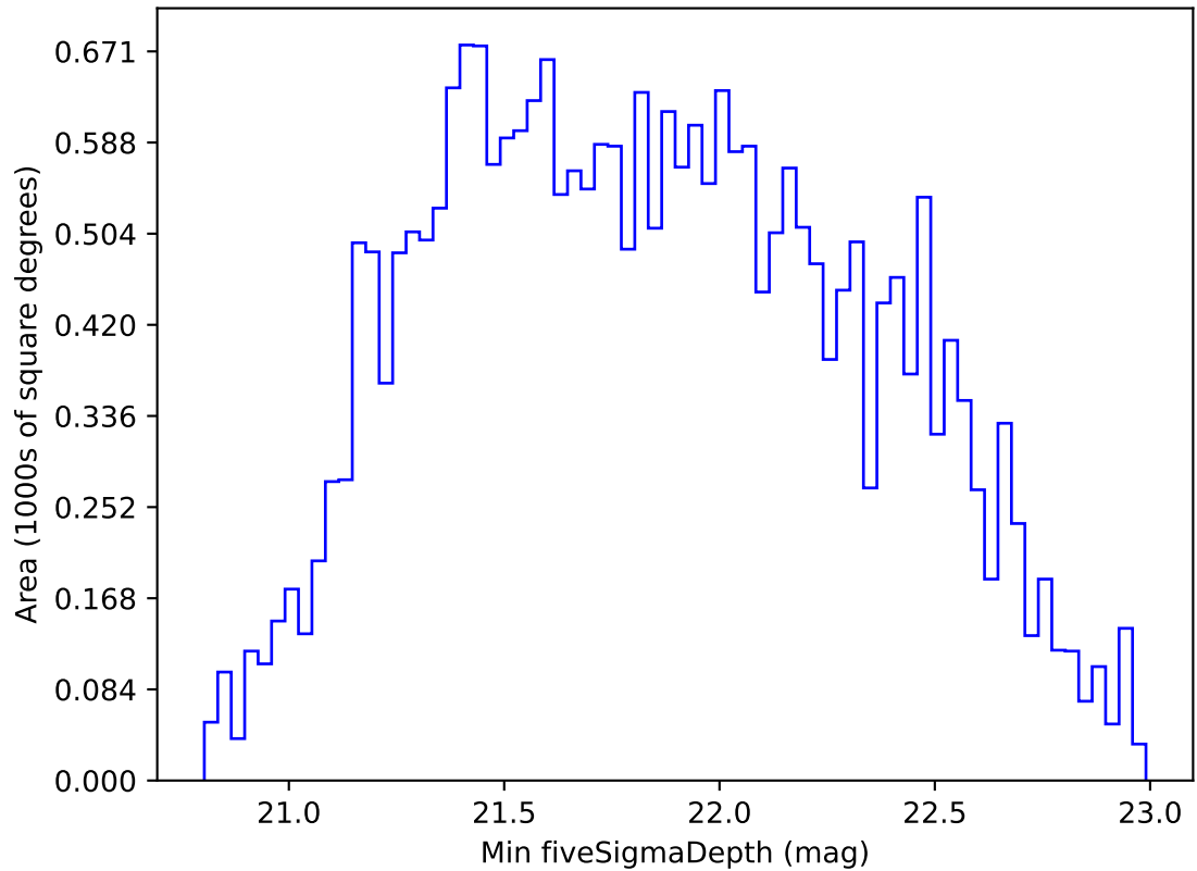
too_elab_2yr_r128_d3_ugrizy_v3.4_10yrs All sky i band: Min fiveSigmaDepth
