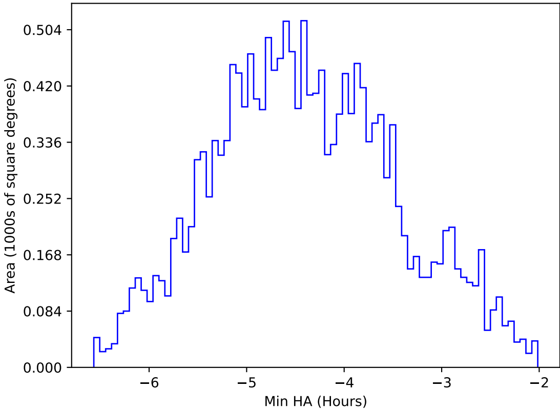
too_elab_2yr_r128_d3_ugrizy_v3.4_10yrs WFD z band: Min HA
