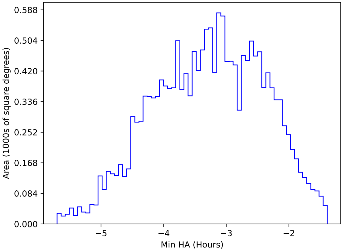
too_elab_2yr_r128_d3_ugrizy_v3.4_10yrs WFD u band: Min HA
