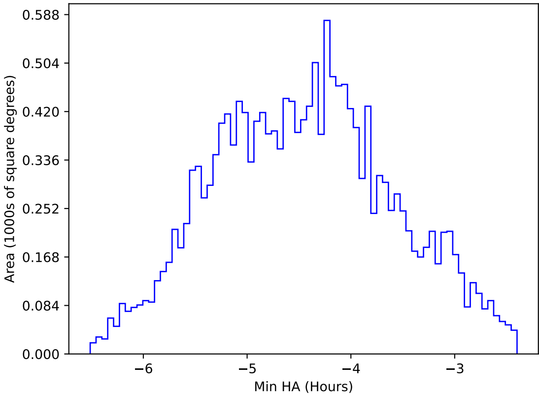
too_elab_2yr_r128_d3_ugrizy_v3.4_10yrs WFD r band: Min HA
