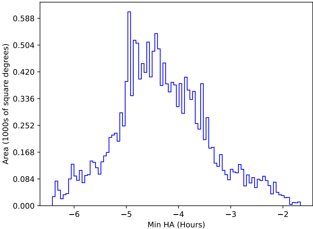
too_elab_2yr_r128_d3_ugrizy_v3.4_10yrs WFD g band: Min HA
