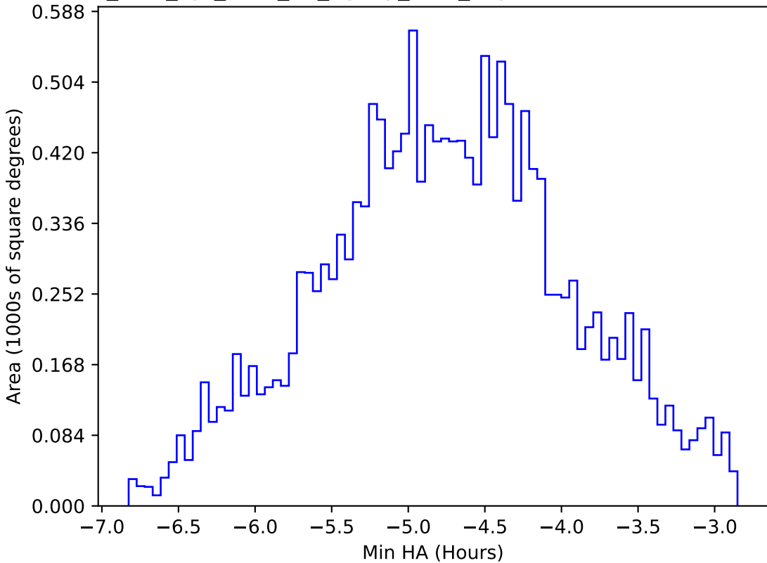
too_elab_2yr_r128_d3_ugrizy_v3.4_10yrs WFD all bands: Min HA
