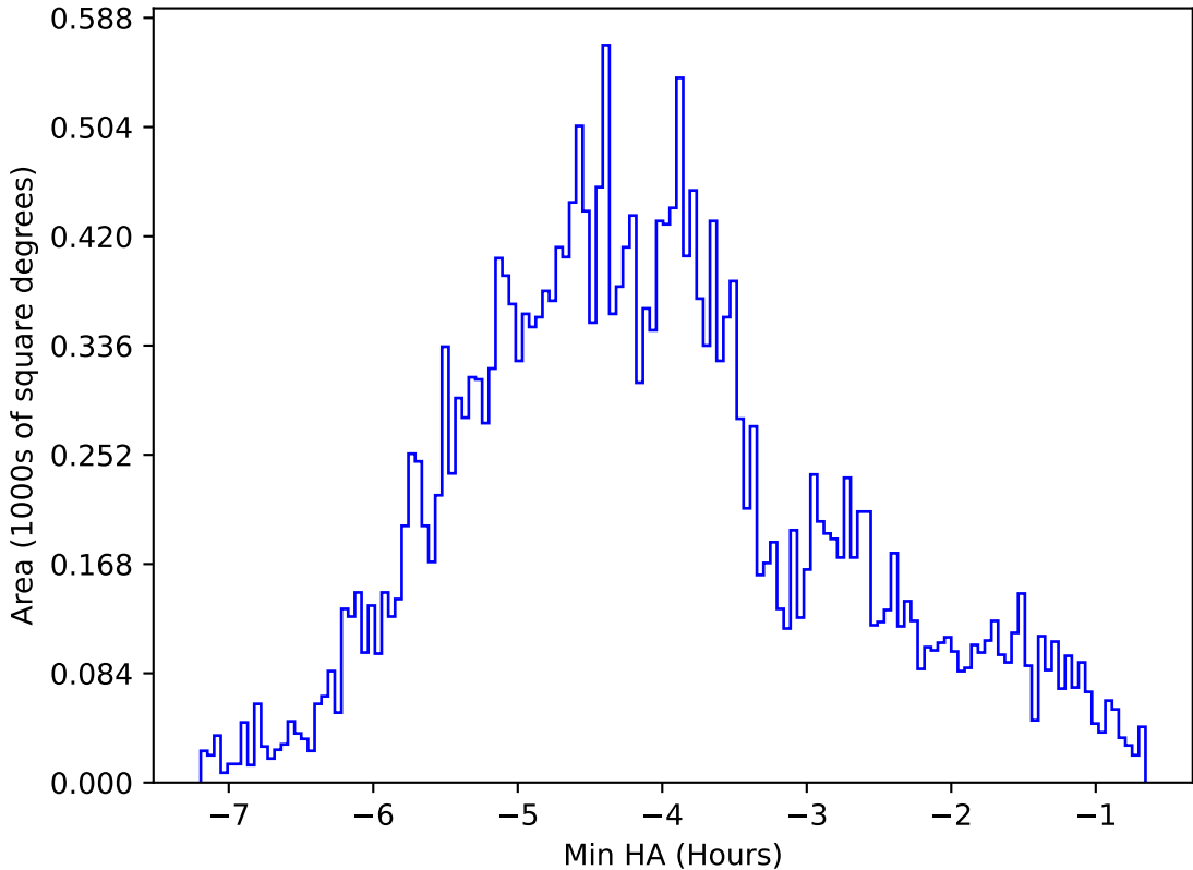
too_elab_2yr_r128_d3_ugrizy_v3.4_10yrs All sky z band: Min HA
