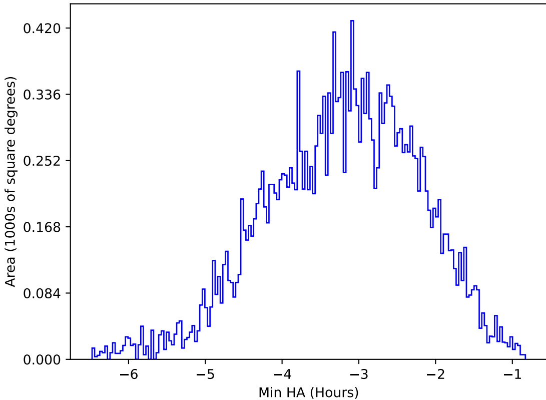
too_elab_2yr_r128_d3_ugrizy_v3.4_10yrs All sky u band: Min HA
