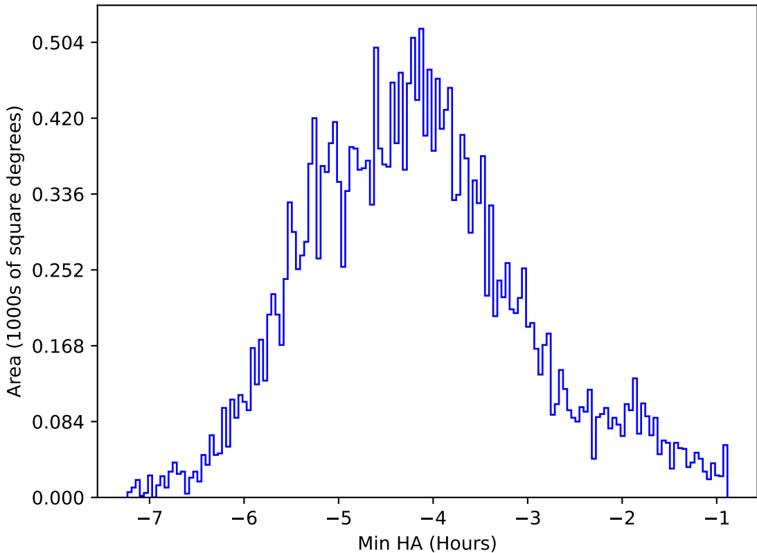
too_elab_2yr_r128_d3_ugrizy_v3.4_10yrs All sky r band: Min HA
