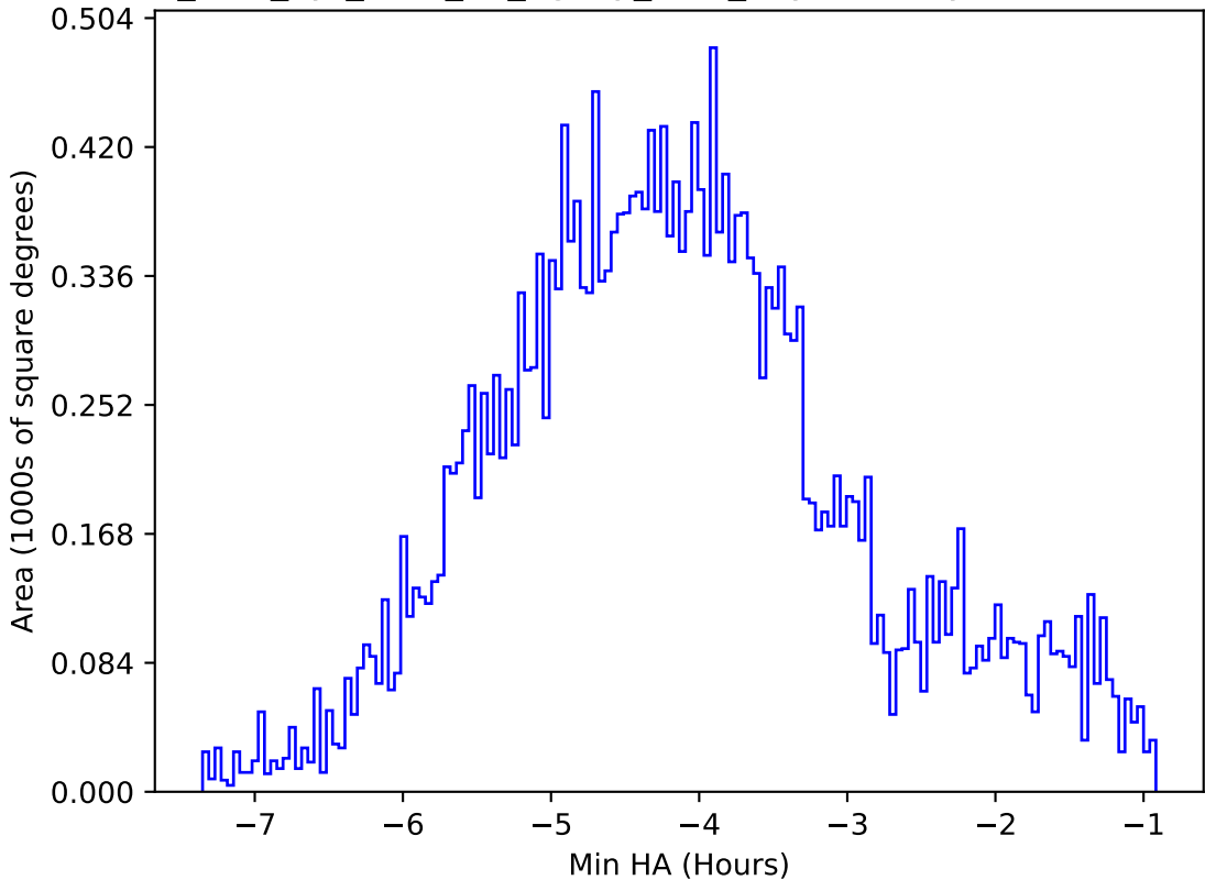
too_elab_2yr_r128_d3_ugrizy_v3.4_10yrs All sky i band: Min HA
