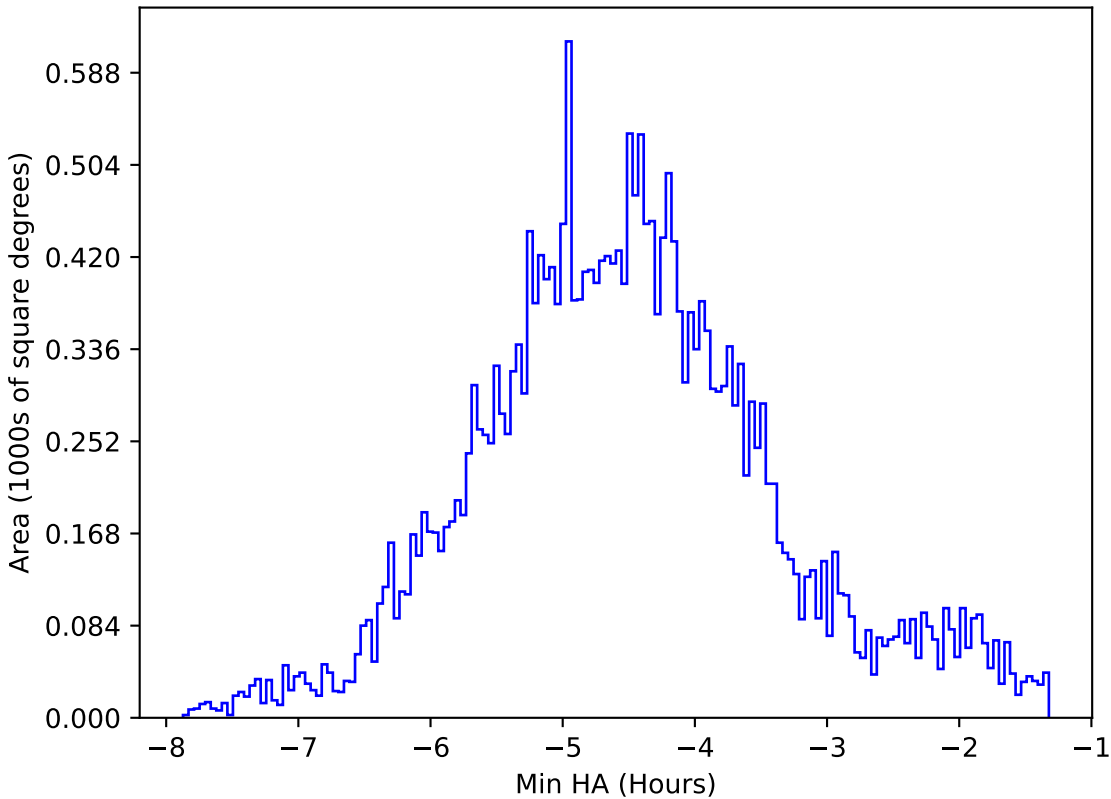
too_elab_2yr_r128_d3_ugrizy_v3.4_10yrs All sky all bands: Min HA
