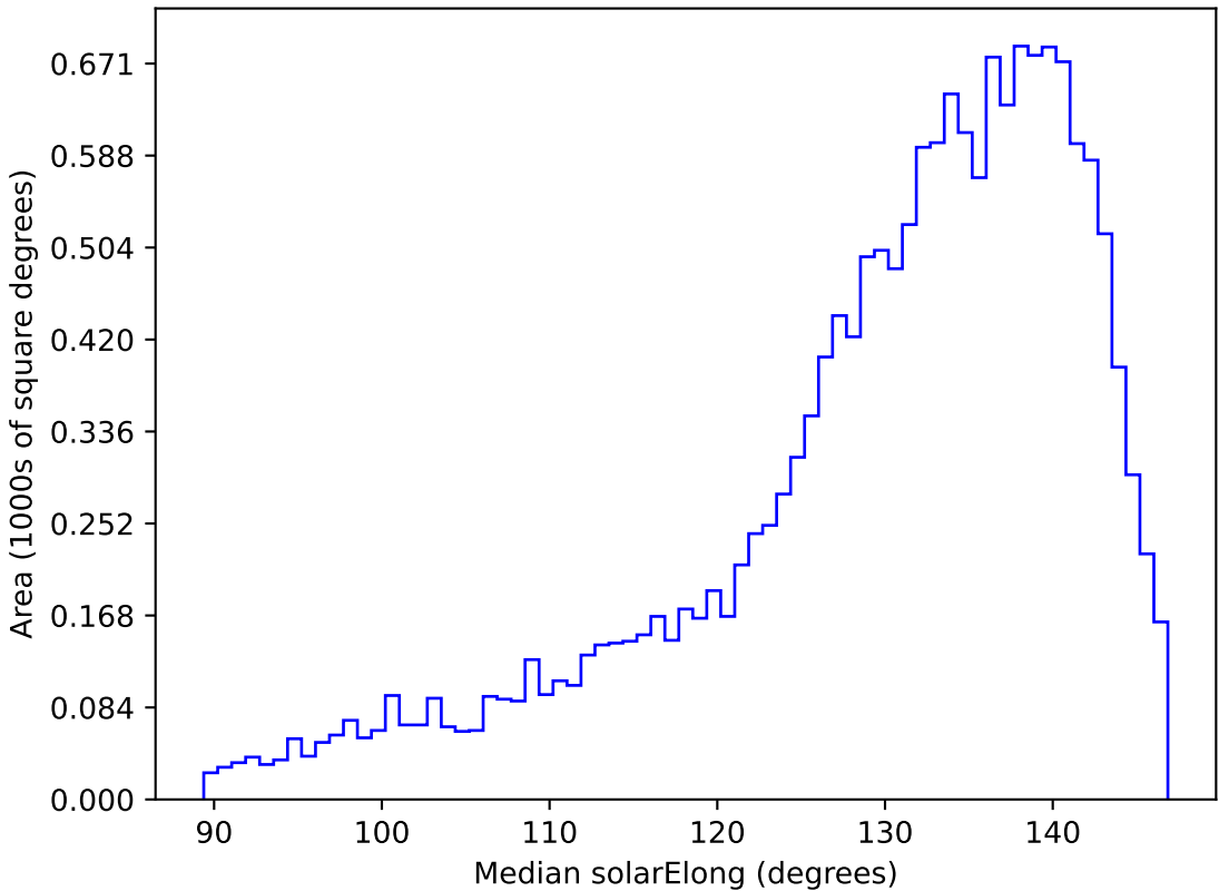
too_elab_2yr_r128_d3_ugrizy_v3.4_10yrs WFD y band: Median solarElong
