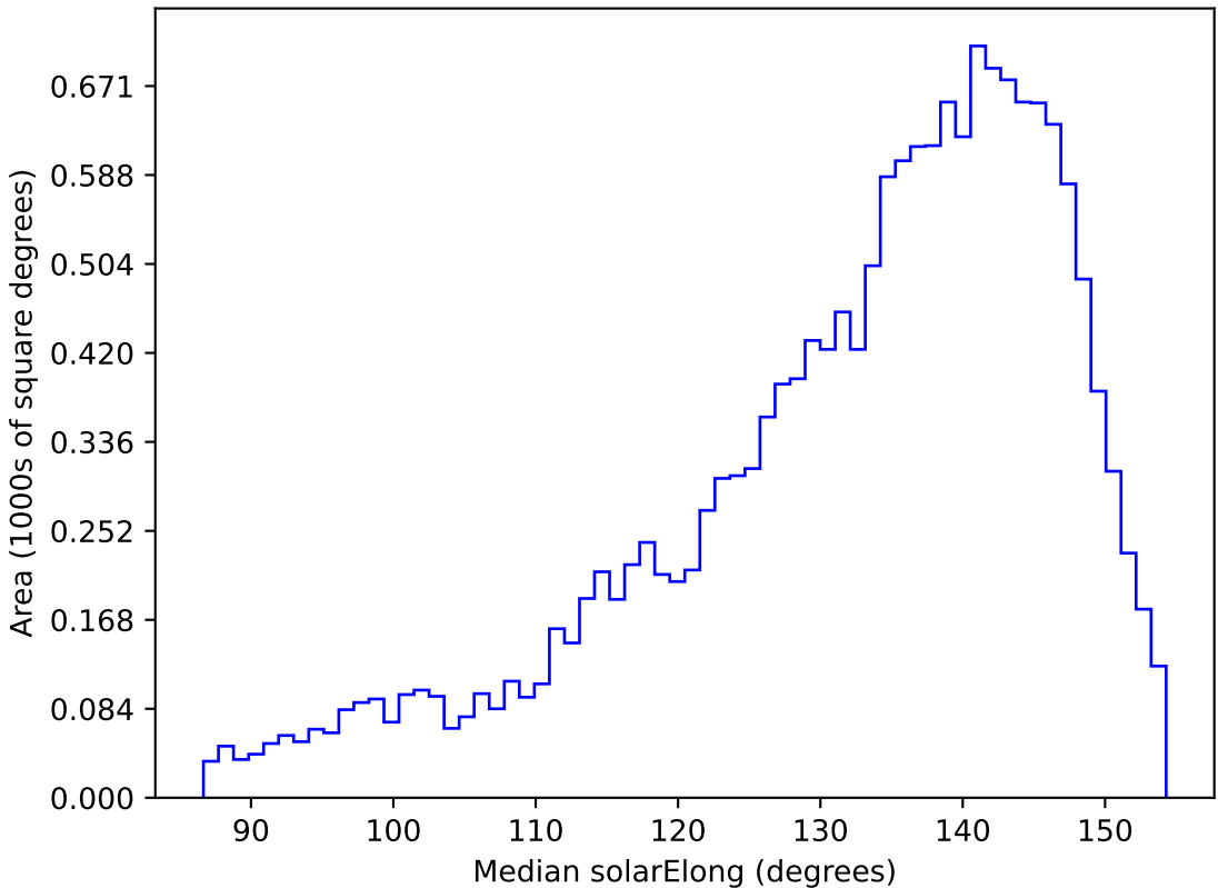
too_elab_2yr_r128_d3_ugrizy_v3.4_10yrs WFD u band: Median solarElong
