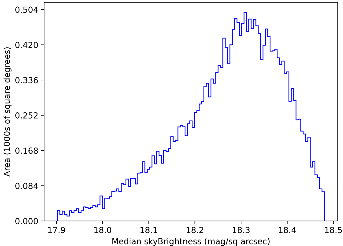
too_elab_2yr_r128_d3_ugrizy_v3.4_10yrs Yr 1 y band: Median skyBrightness
