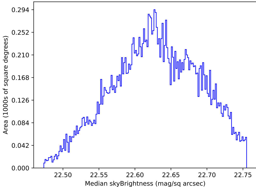
too_elab_2yr_r128_d3_ugrizy_v3.4_10yrs Yr 1 u band: Median skyBrightness
