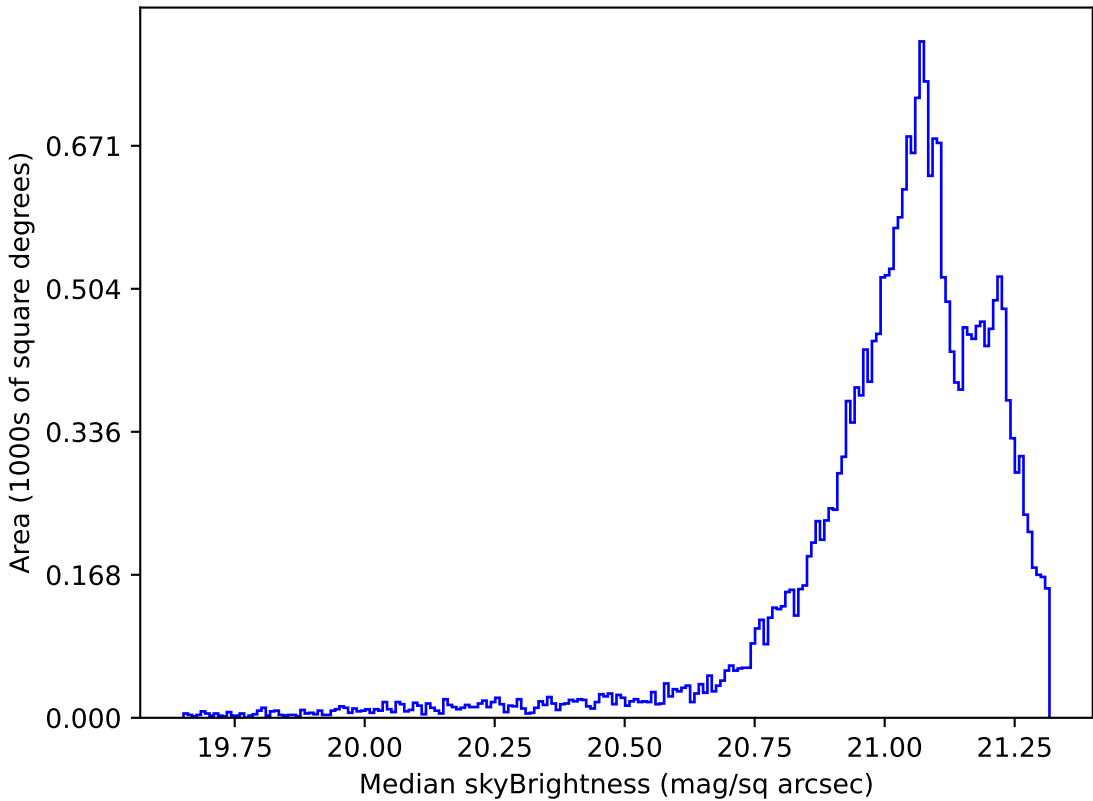
too_elab_2yr_r128_d3_ugrizy_v3.4_10yrs Yr 1 r band: Median skyBrightness
