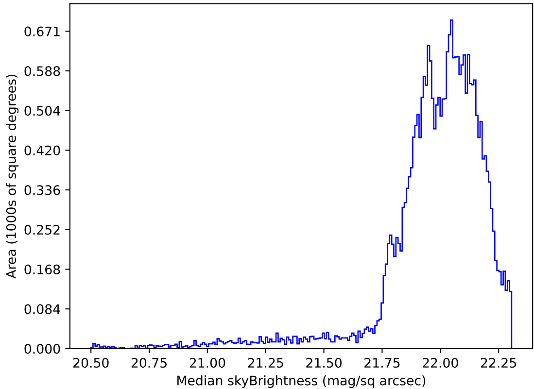
too_elab_2yr_r128_d3_ugrizy_v3.4_10yrs Yr 1 g band: Median skyBrightness
