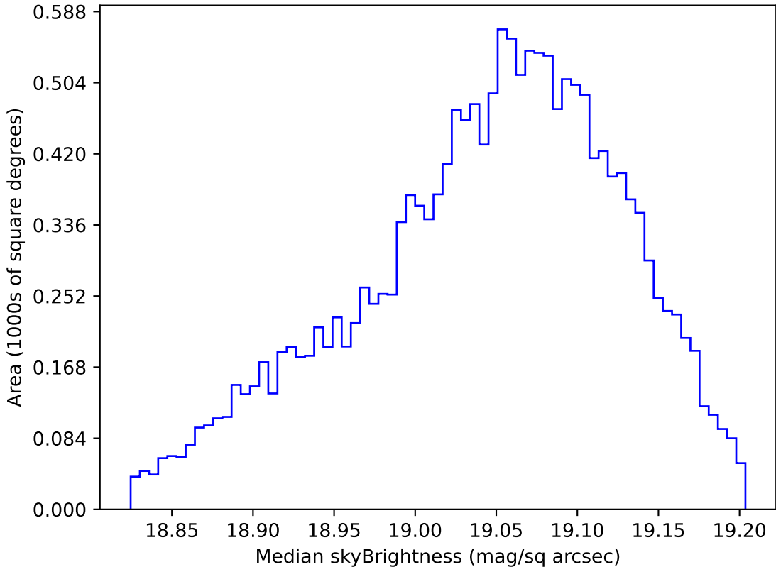
too_elab_2yr_r128_d3_ugrizy_v3.4_10yrs WFD z band: Median skyBrightness
