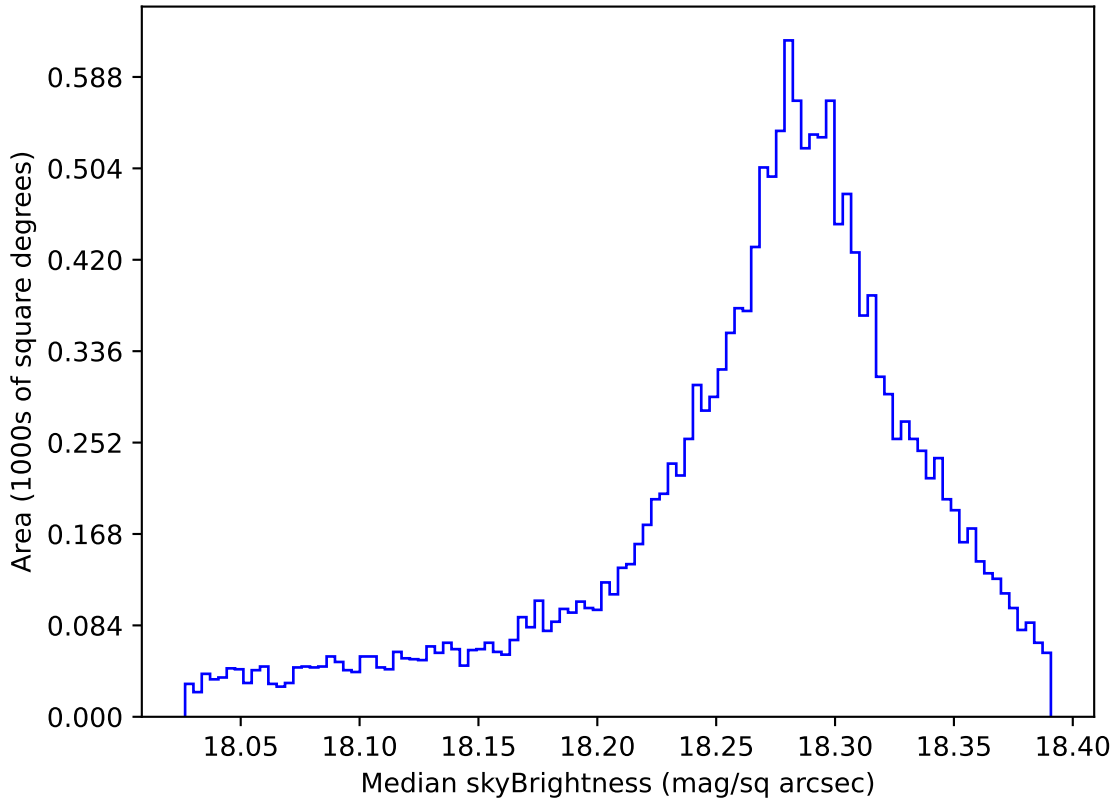
too_elab_2yr_r128_d3_ugrizy_v3.4_10yrs WFD y band: Median skyBrightness
