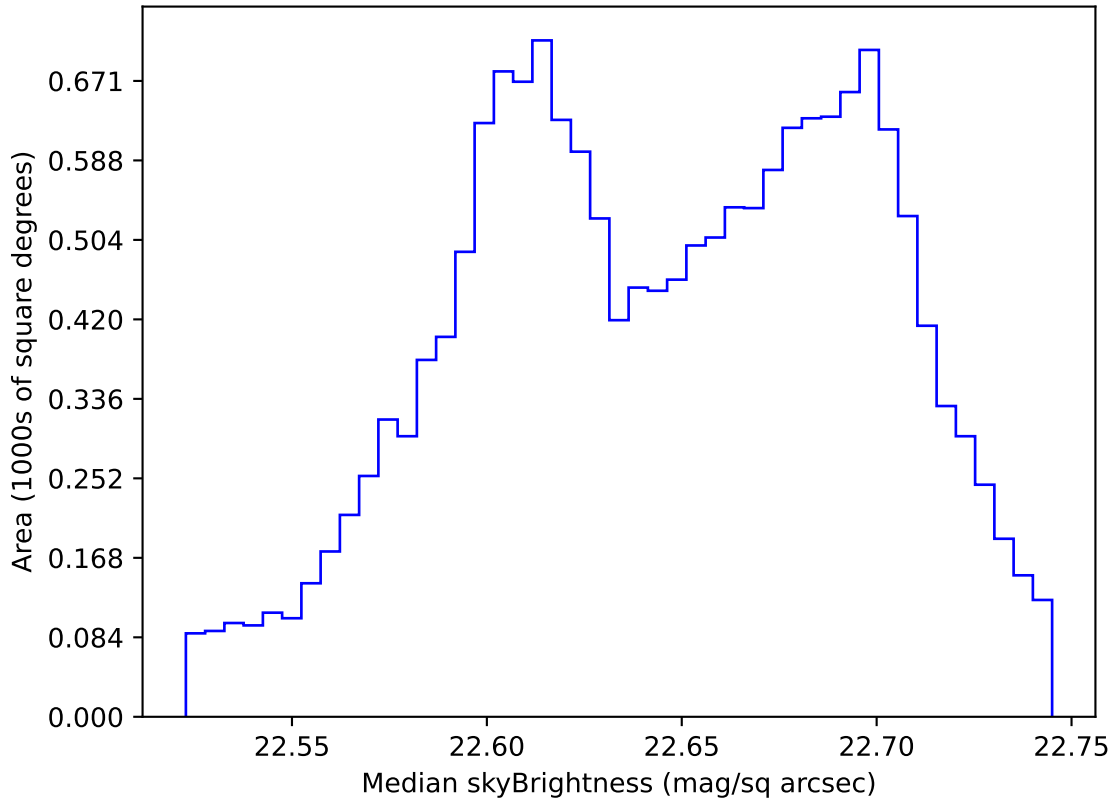
too_elab_2yr_r128_d3_ugrizy_v3.4_10yrs WFD u band: Median skyBrightness
