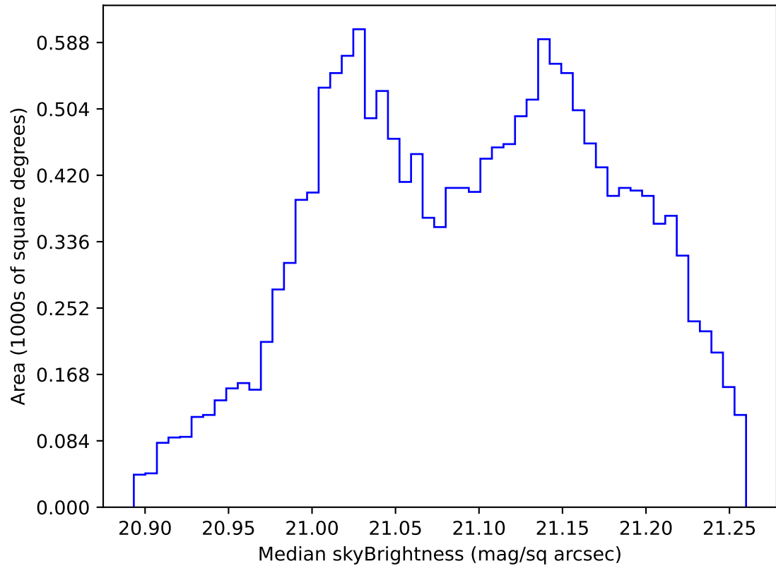
too_elab_2yr_r128_d3_ugrizy_v3.4_10yrs WFD r band: Median skyBrightness
