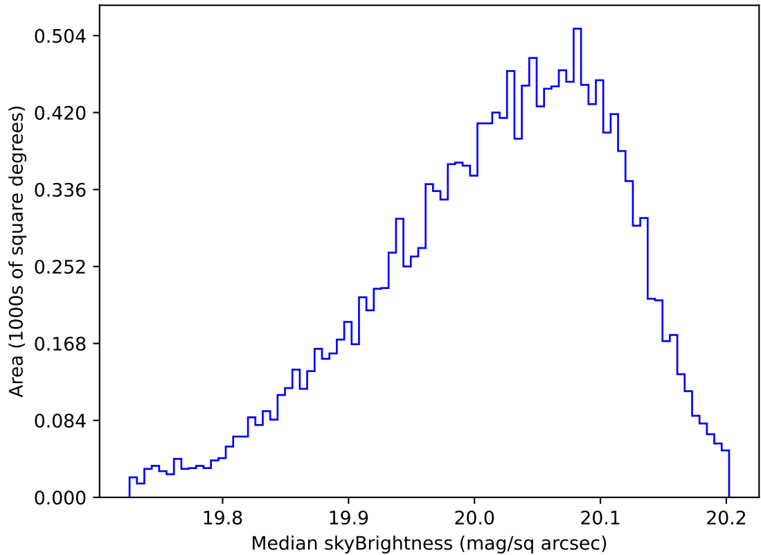
too_elab_2yr_r128_d3_ugrizy_v3.4_10yrs WFD i band: Median skyBrightness
